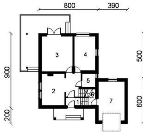
Parter
