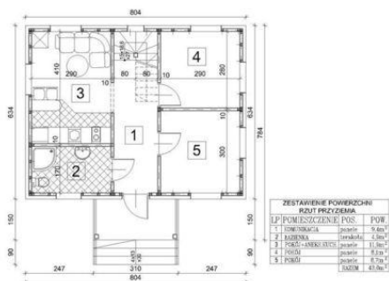
Parter
