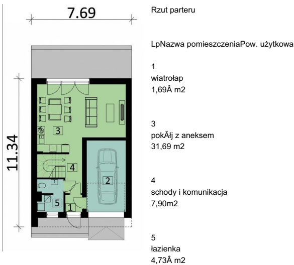
Parter
